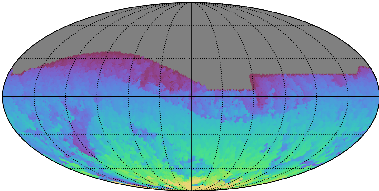
smc_lmc_v3.3_10yrs All sky z band: Max HA
