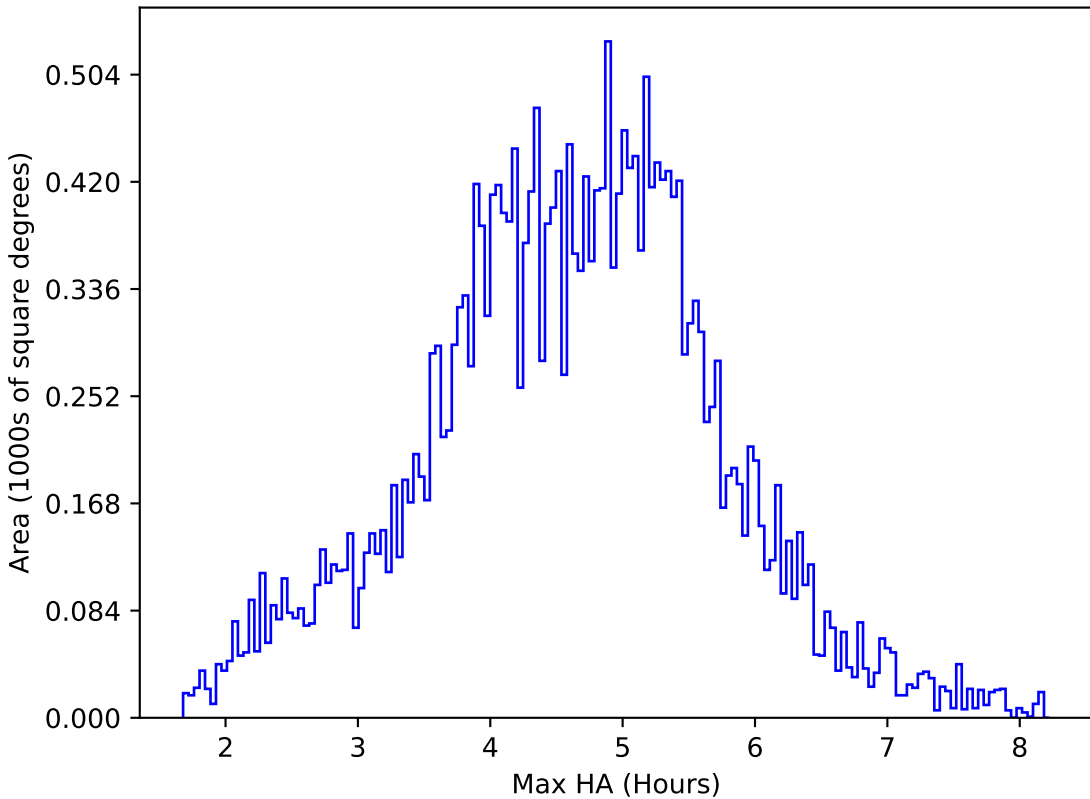
smc_lmc_v3.3_10yrs All sky z band: Max HA
