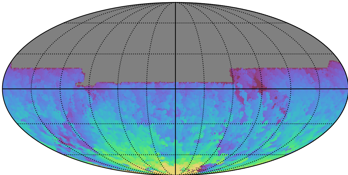
smc_lmc_v3.3_10yrs All sky y band: Max HA
