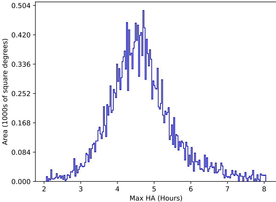
smc_lmc_v3.3_10yrs All sky y band: Max HA
