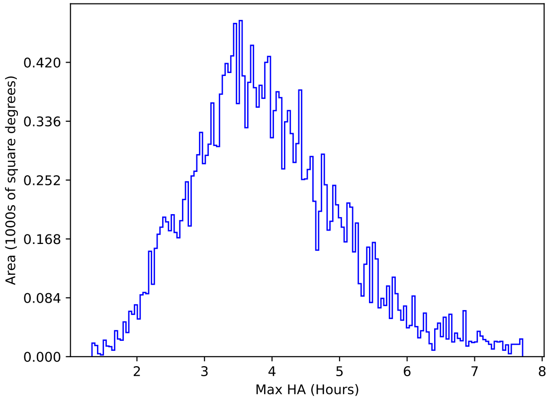
smc_lmc_v3.3_10yrs All sky u band: Max HA
