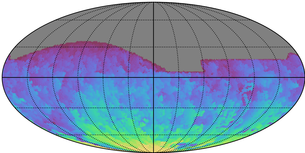
smc_lmc_v3.3_10yrs All sky r band: Max HA
