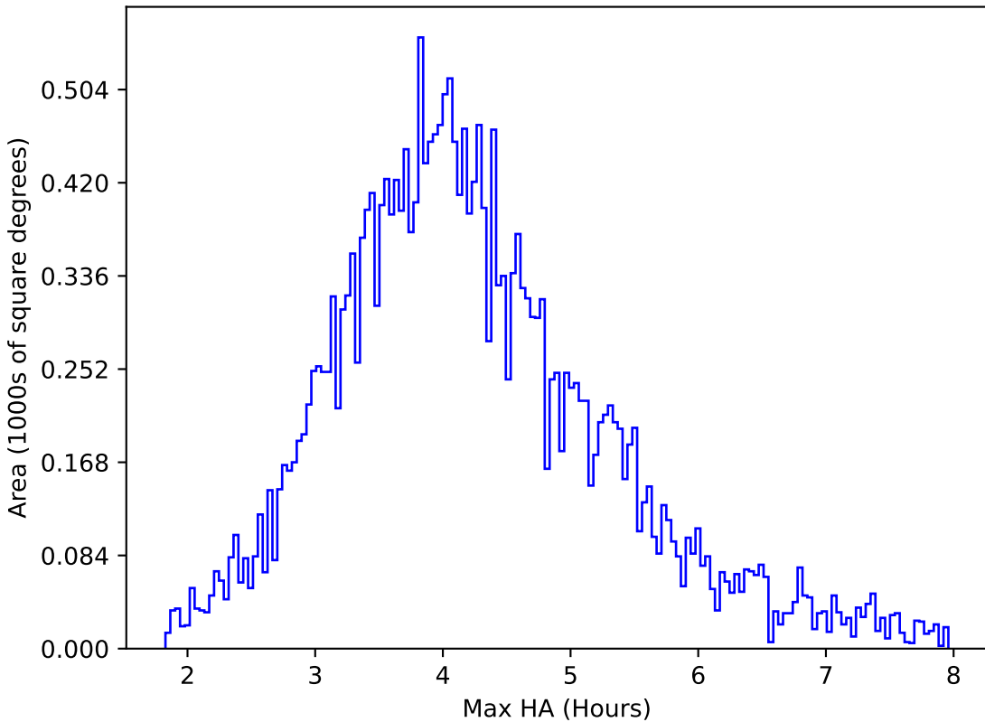
smc_lmc_v3.3_10yrs All sky r band: Max HA
