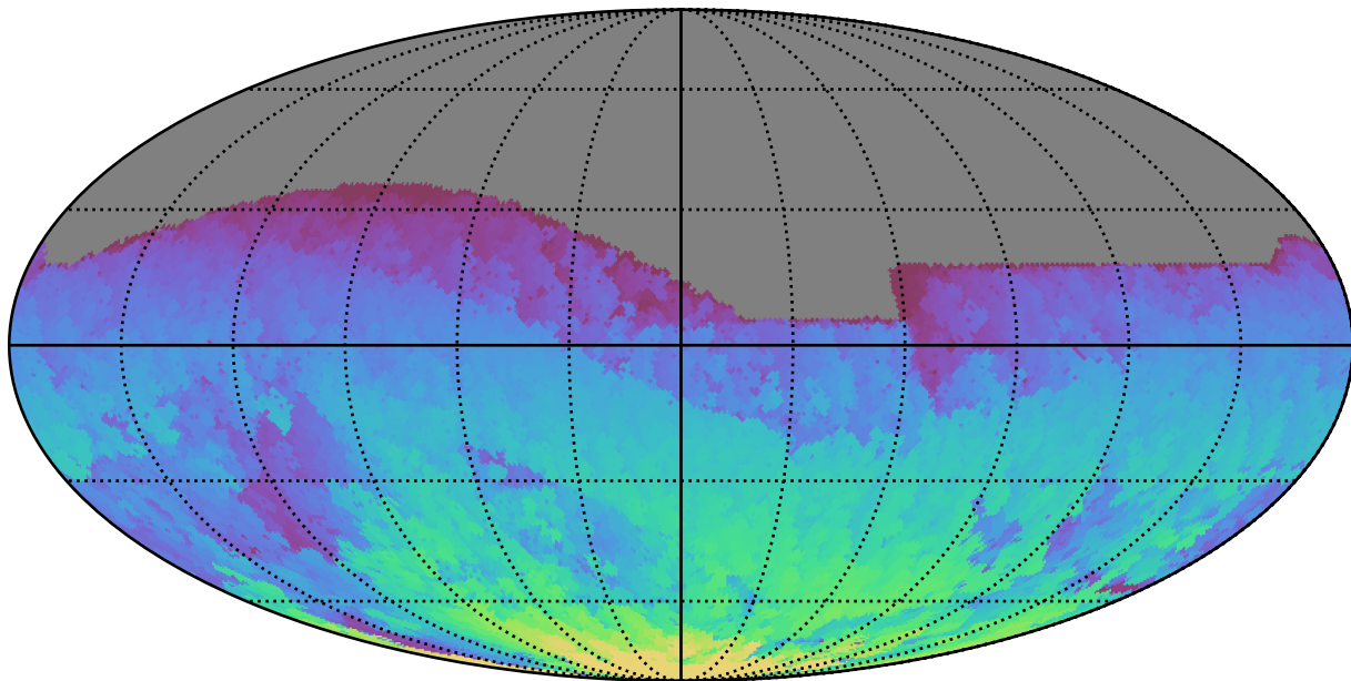
smc_lmc_v3.3_10yrs All sky i band: Max HA
