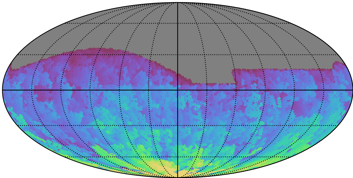
smc_lmc_v3.3_10yrs All sky g band: Max HA
