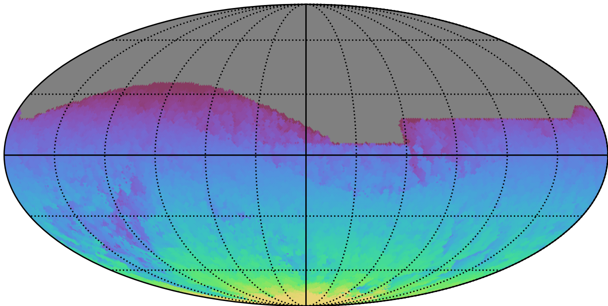
smc_lmc_v3.3_10yrs All sky all bands: Max HA
