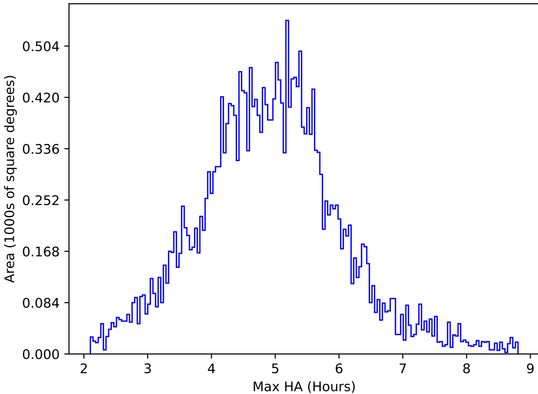
smc_lmc_v3.3_10yrs All sky all bands: Max HA
