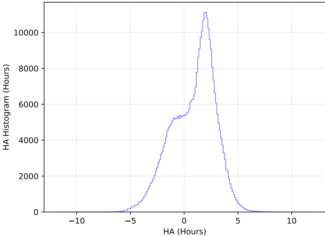
smc_lmc_v3.3_10yrs WFD y band: HA Histogram
