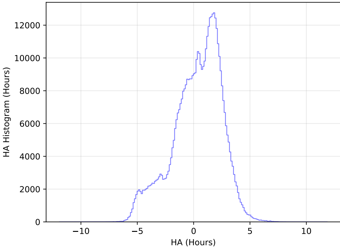
smc_lmc_v3.3_10yrs WFD r band: HA Histogram
