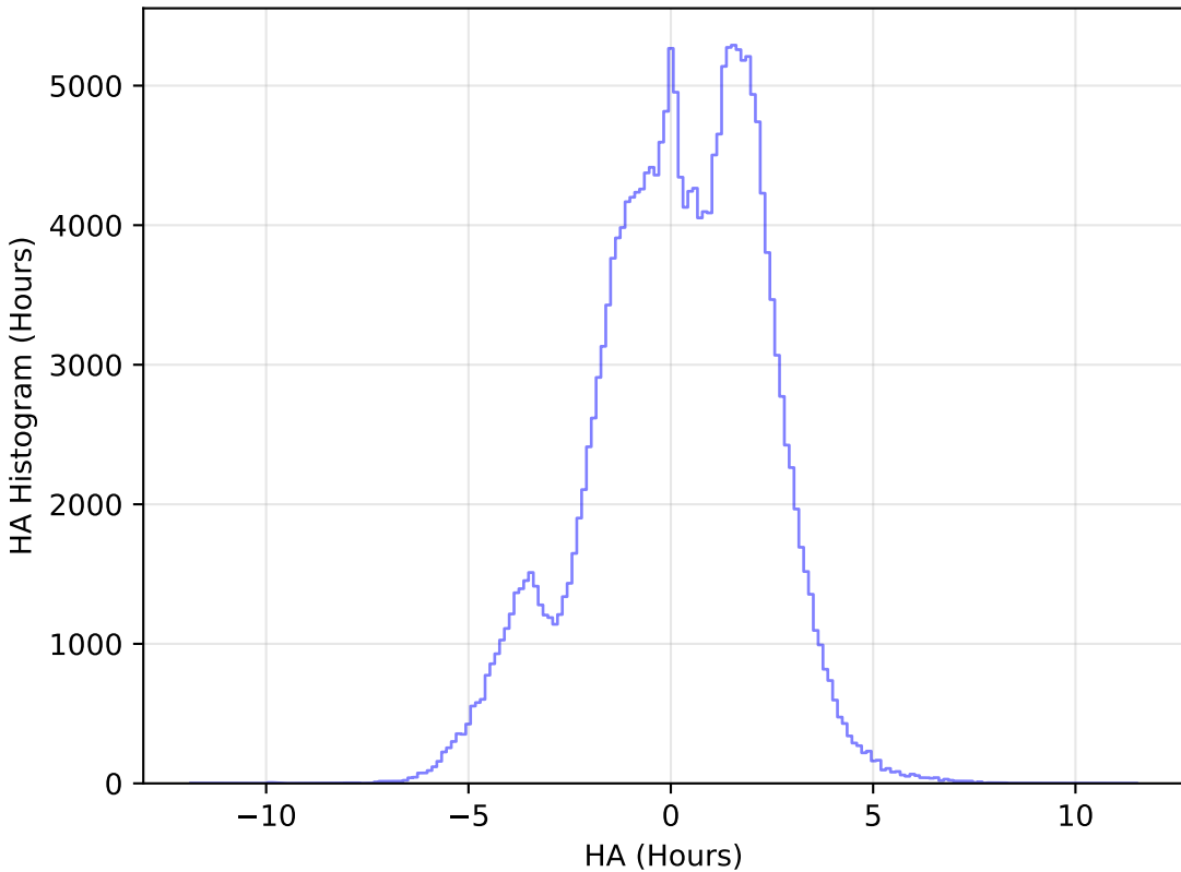
smc_lmc_v3.3_10yrs WFD g band: HA Histogram
