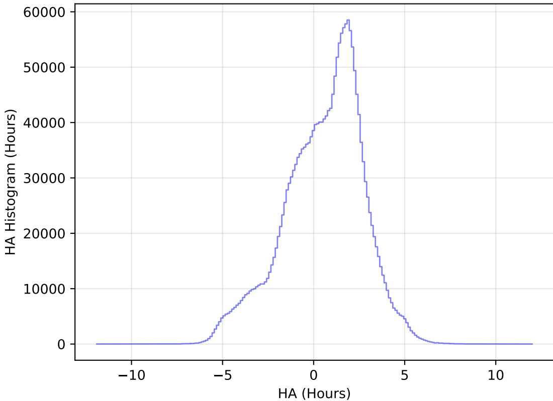
smc_lmc_v3.3_10yrs WFD all bands: HA Histogram
