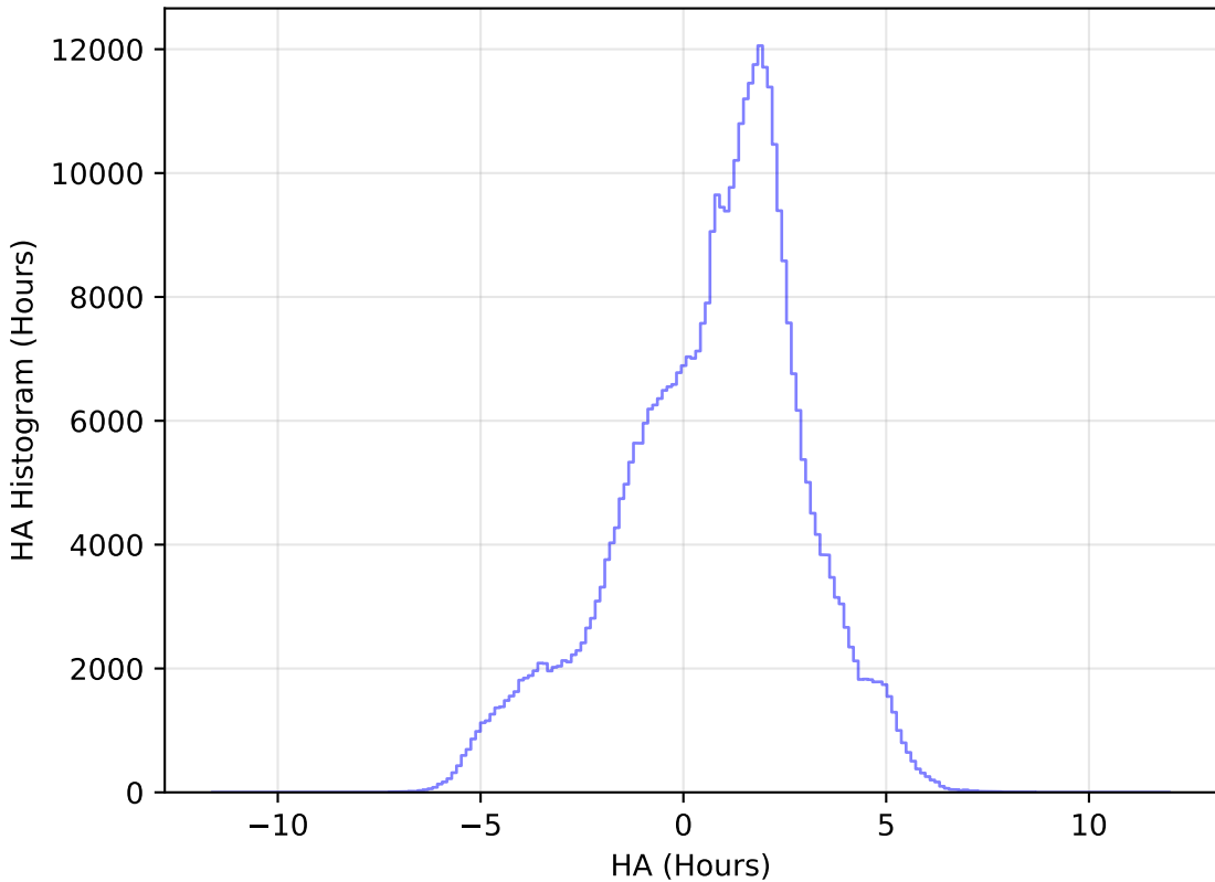
smc_lmc_v3.3_10yrs All sky z band: HA Histogram
