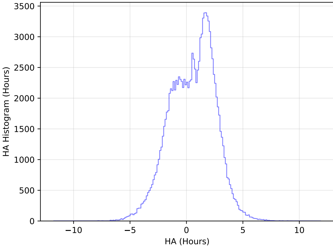
smc_lmc_v3.3_10yrs All sky u band: HA Histogram
