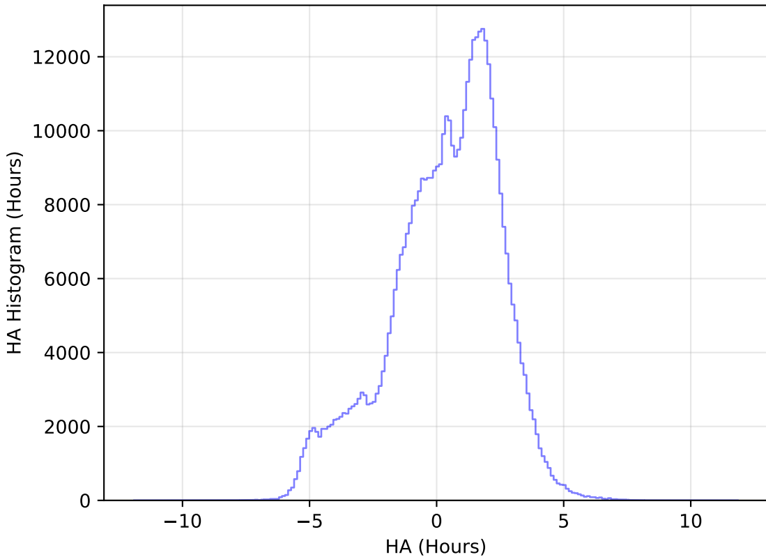
smc_lmc_v3.3_10yrs All sky r band: HA Histogram
