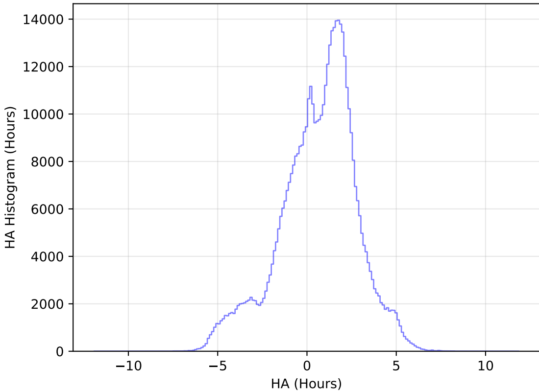
smc_lmc_v3.3_10yrs All sky i band: HA Histogram
