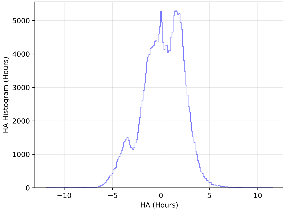
smc_lmc_v3.3_10yrs All sky g band: HA Histogram
