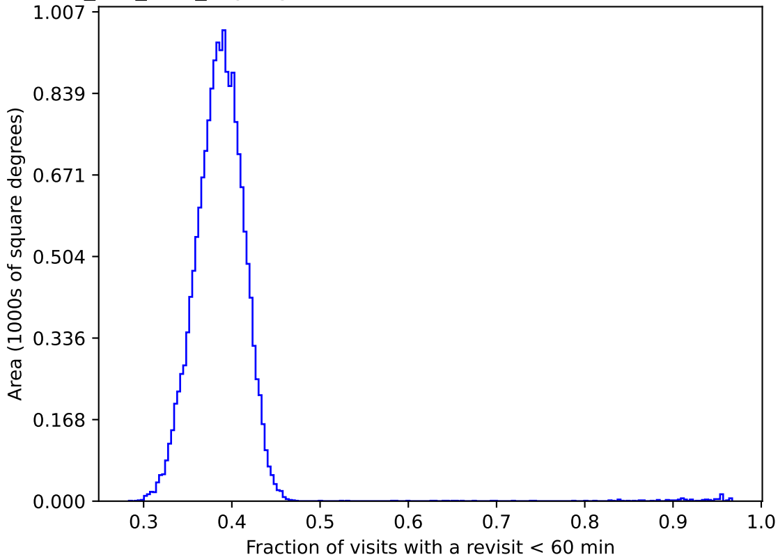
smc_lmc_v3.3_10yrs gri WFD: Fraction of visits with a revisit < 60 min
