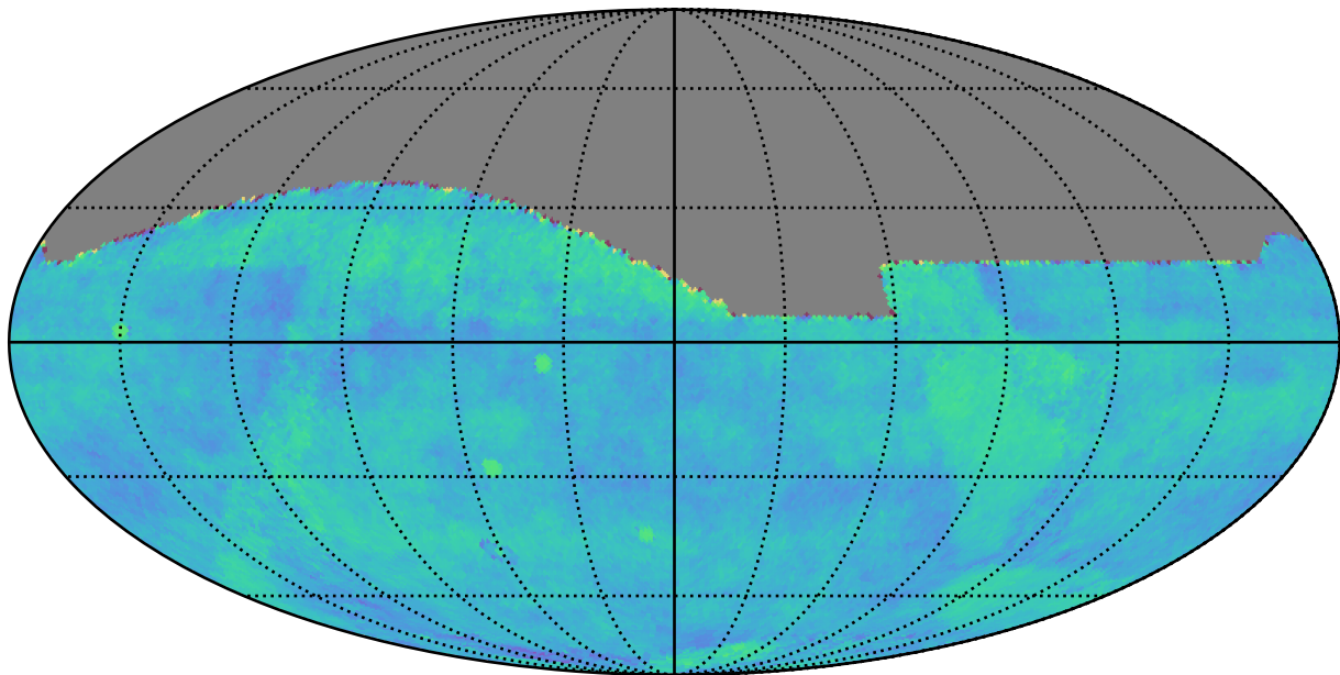
smc_lmc_v3.3_10yrs gri All sky: Fraction of visits in pairs (20-90 min)
