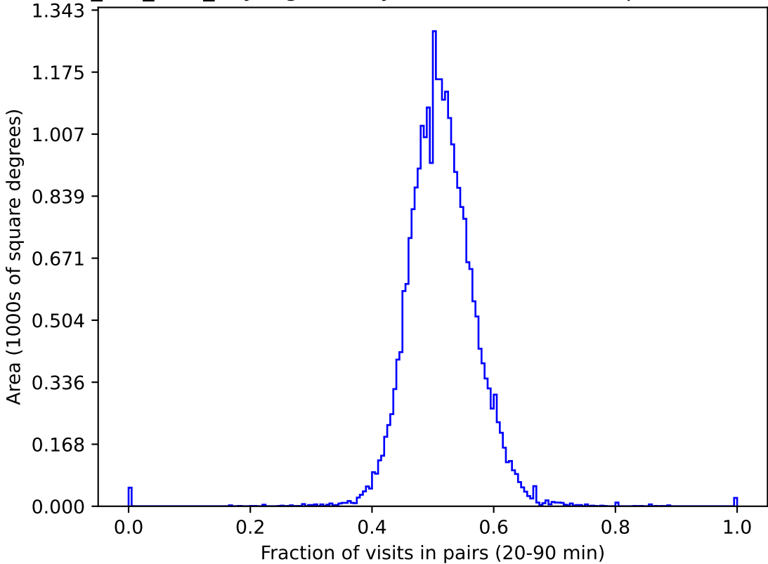
smc_lmc_v3.3_10yrs gri All sky: Fraction of visits in pairs (20-90 min)
