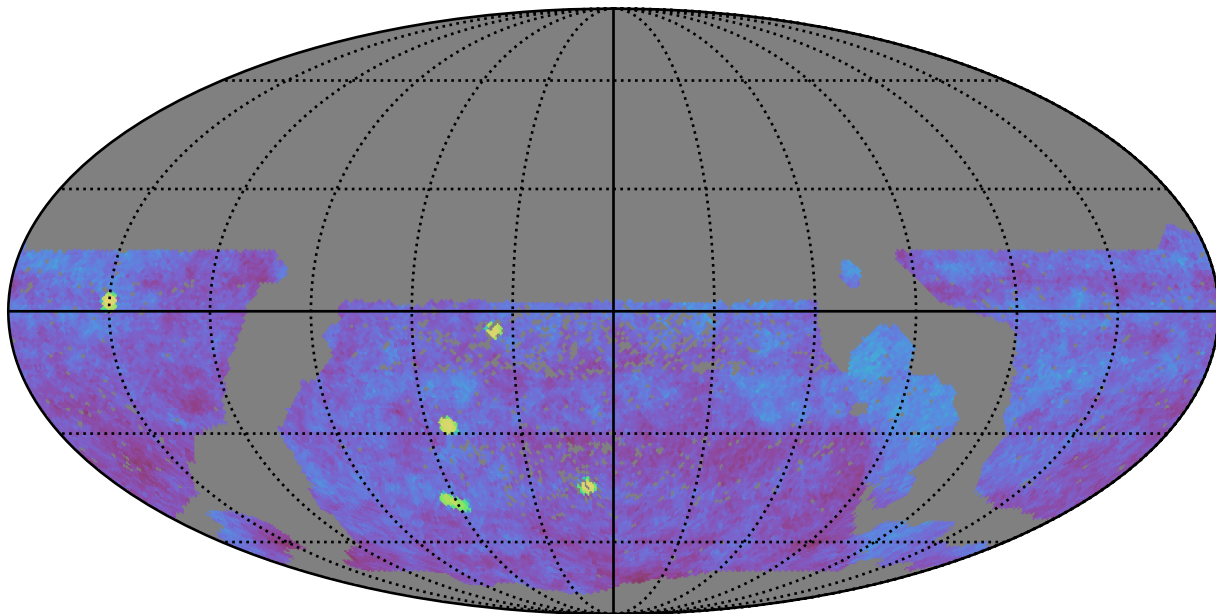
smc_lmc_v3.3_10yrs gri WFD: Fraction of visits in pairs (10-60 min)
