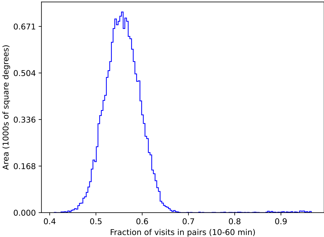
smc_lmc_v3.3_10yrs gri WFD: Fraction of visits in pairs (10-60 min)
