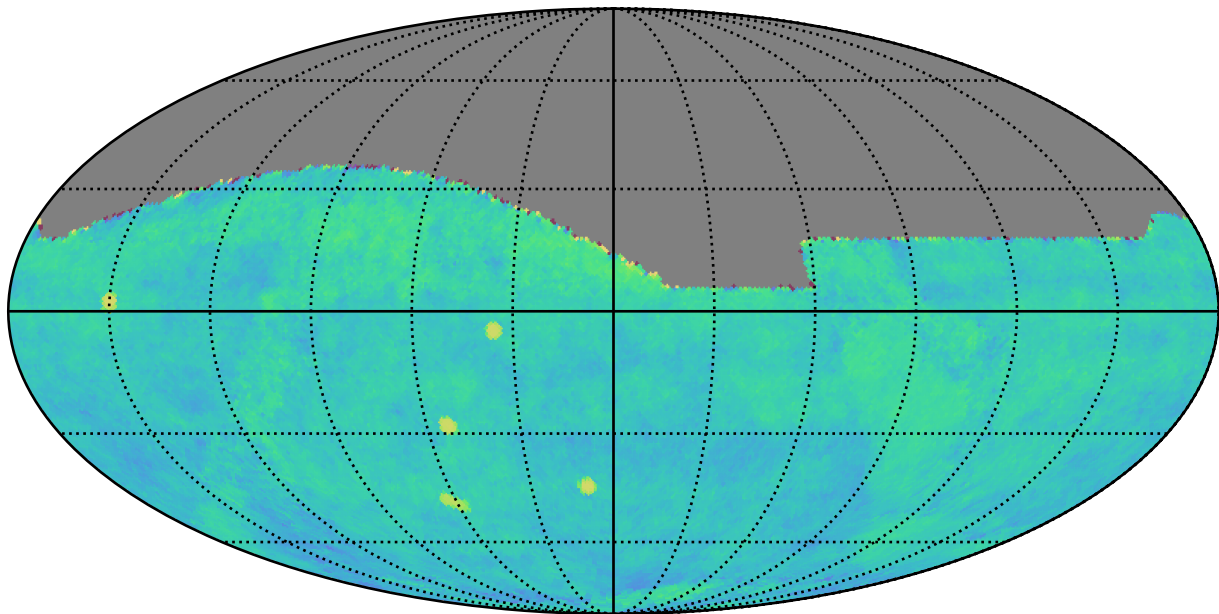
smc_lmc_v3.3_10yrs gri All sky: Fraction of visits in pairs (10-60 min)
