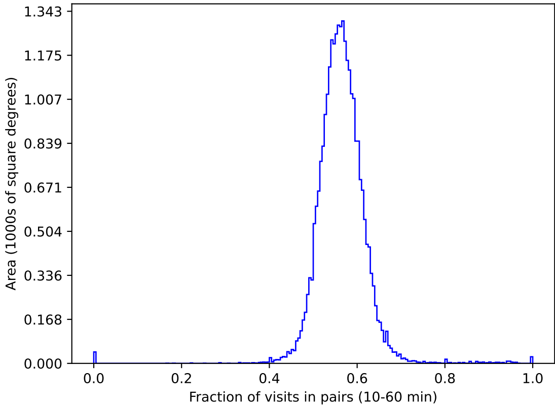
smc_lmc_v3.3_10yrs gri All sky: Fraction of visits in pairs (10-60 min)
