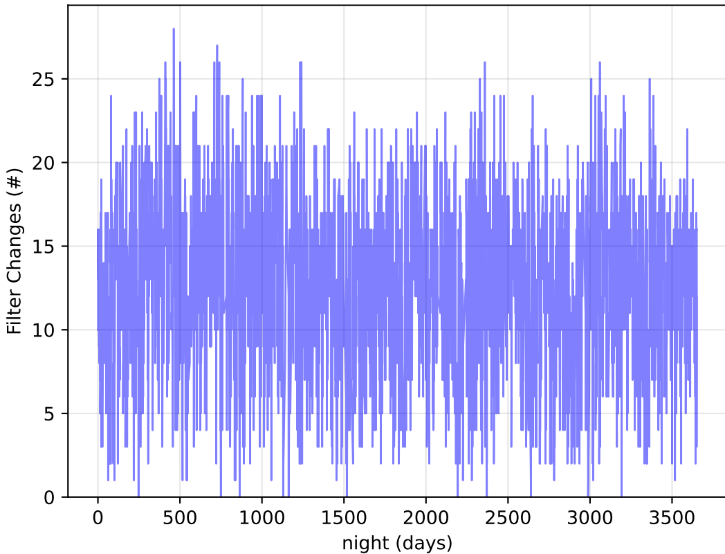
smc_lmc_v3.3_10yrs Per Night: Filter Changes
