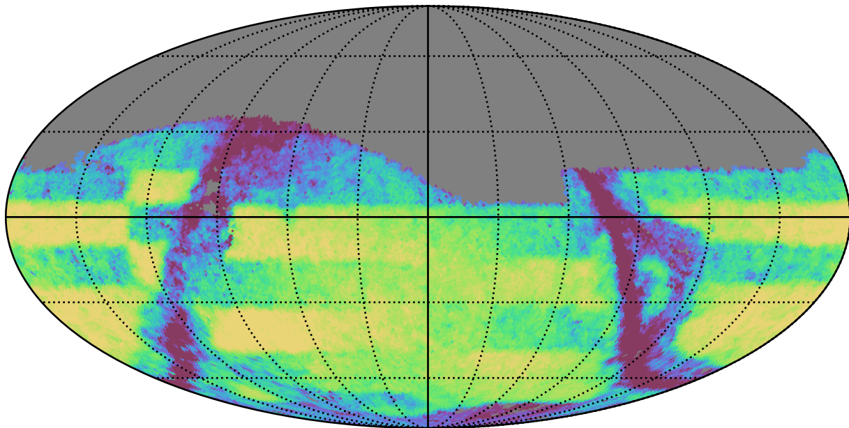
smc_lmc_v3.3_10yrs Yr 3-4 z band: Exgal_CoaddM5
