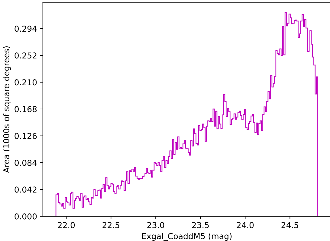
smc_lmc_v3.3_10yrs Yr 3-4 z band: Exgal_CoaddM5
