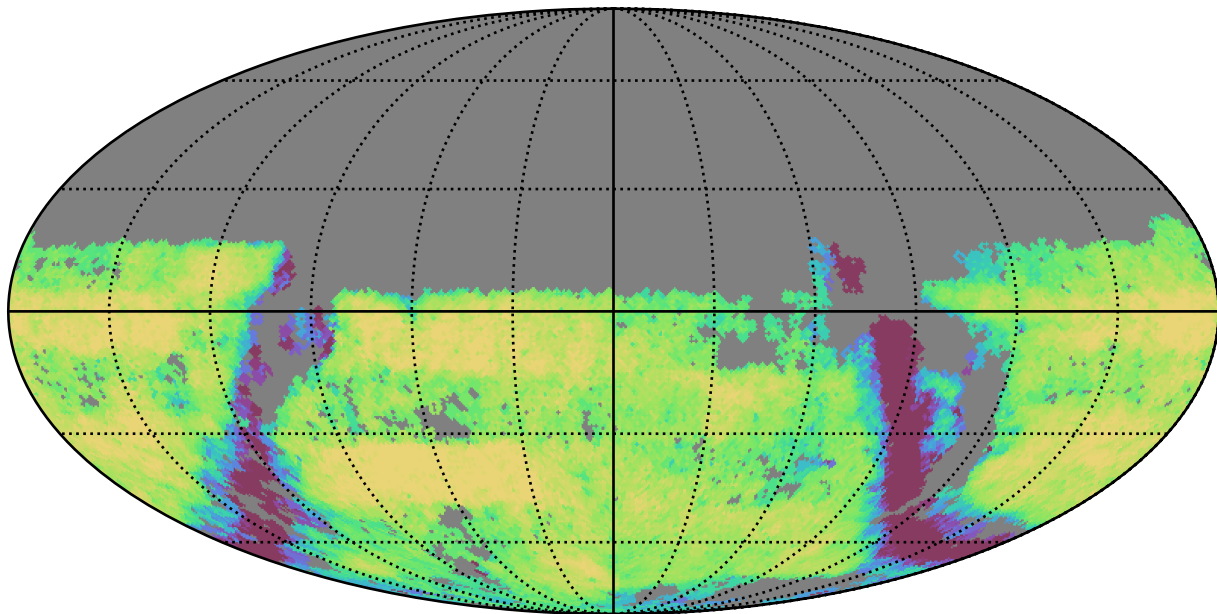
smc_lmc_v3.3_10yrs Yr 3-4 u band: Exgal_CoaddM5
