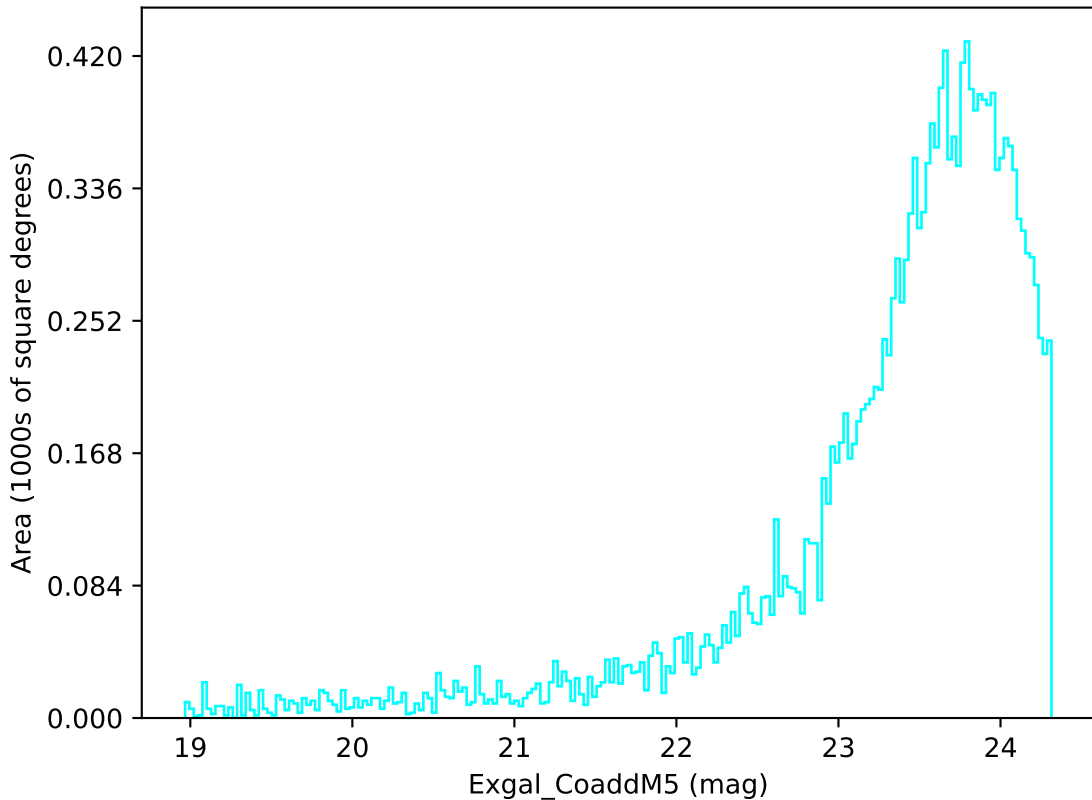
smc_lmc_v3.3_10yrs Yr 3-4 u band: Exgal_CoaddM5
