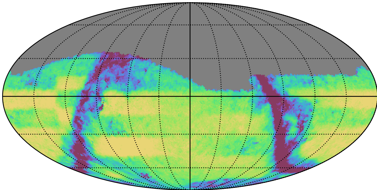
smc_lmc_v3.3_10yrs Yr 3-4 r band: Exgal_CoaddM5
