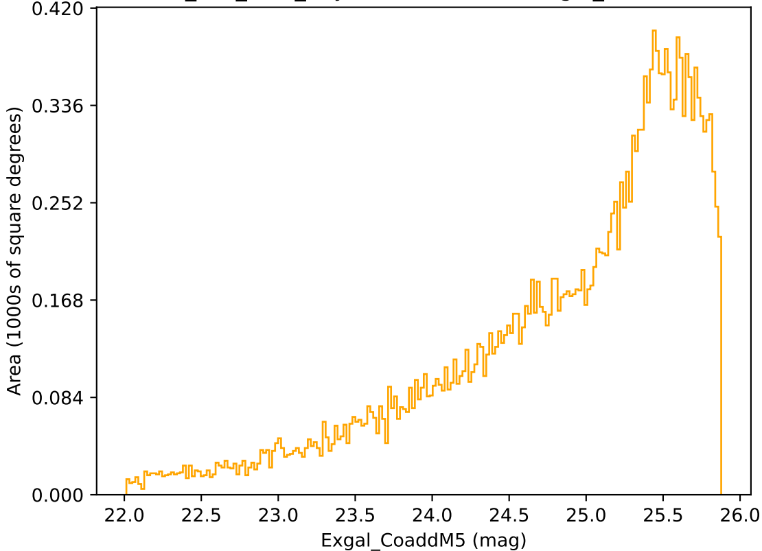
smc_lmc_v3.3_10yrs Yr 3-4 r band: Exgal_CoaddM5
