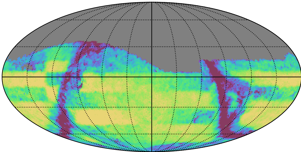
smc_lmc_v3.3_10yrs Yr 3-4 i band: Exgal_CoaddM5
