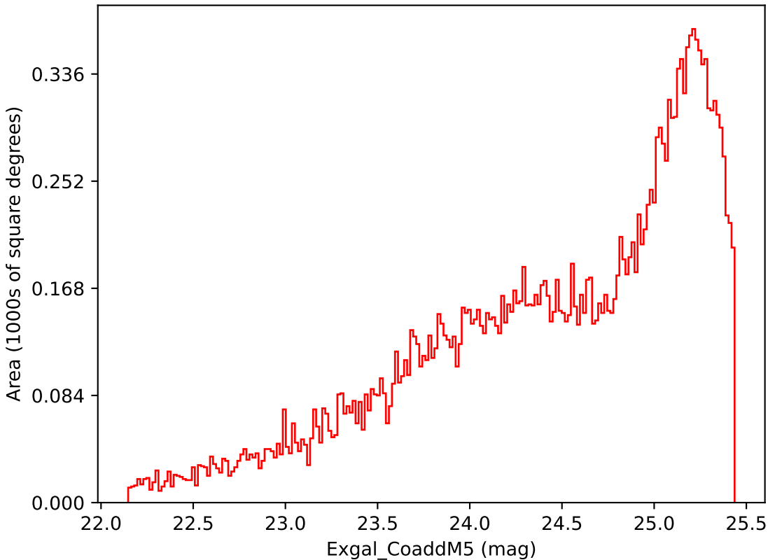
smc_lmc_v3.3_10yrs Yr 3-4 i band: Exgal_CoaddM5
