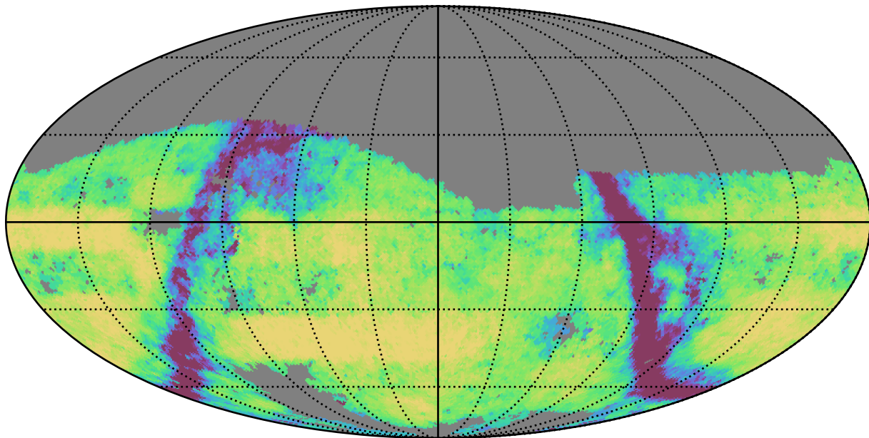
smc_lmc_v3.3_10yrs Yr 3-4 g band: Exgal_CoaddM5
