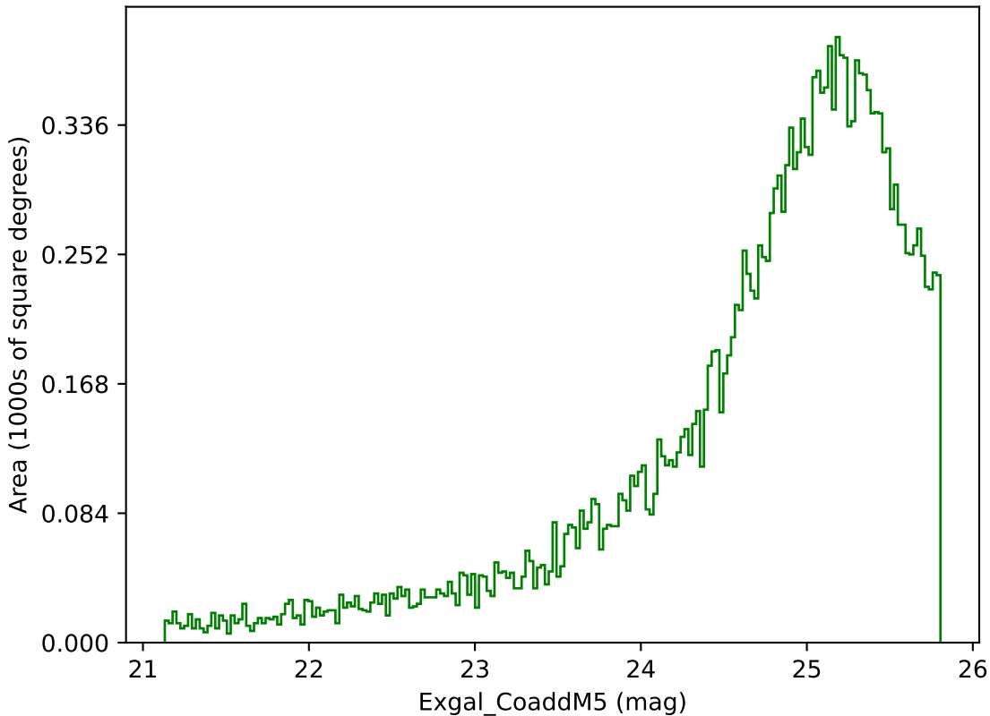
smc_lmc_v3.3_10yrs Yr 3-4 g band: Exgal_CoaddM5
