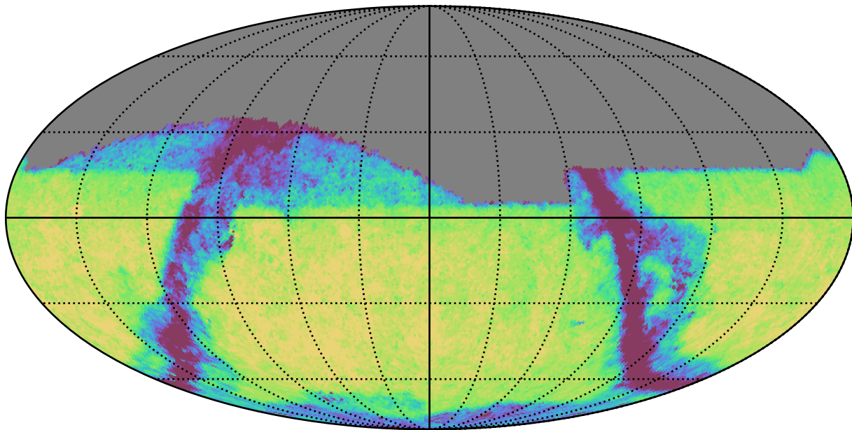
smc_lmc_v3.3_10yrs Yr 1 z band: Exgal_CoaddM5
