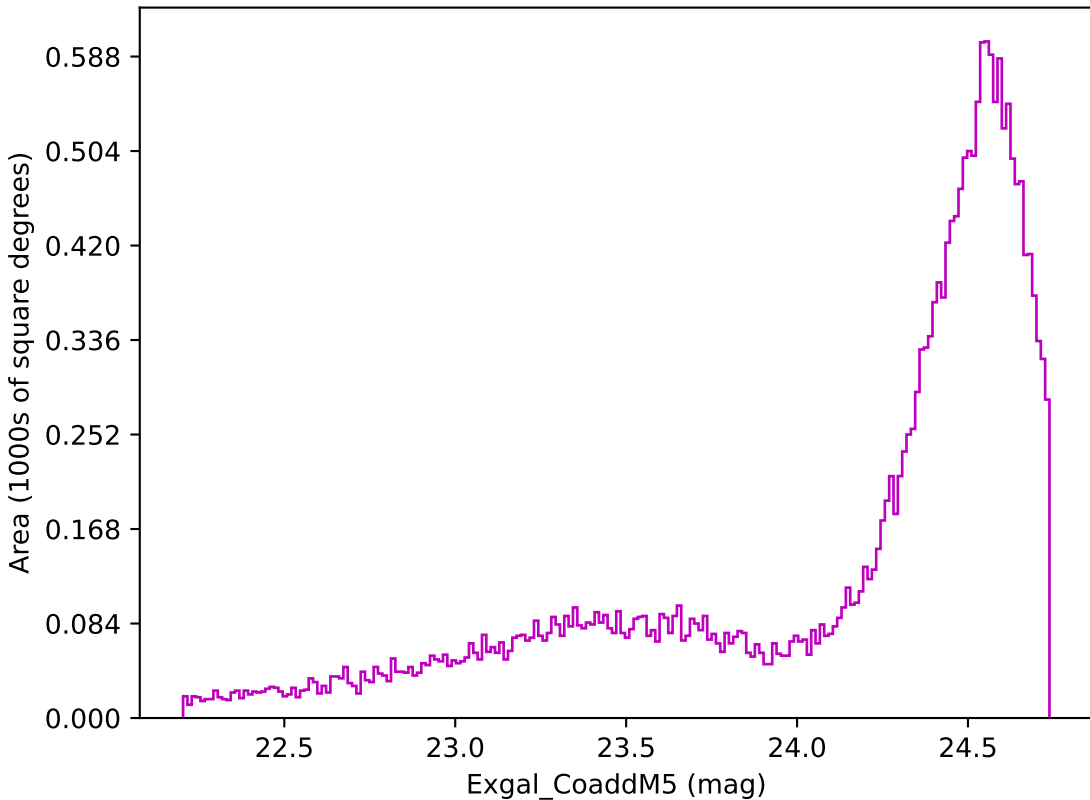
smc_lmc_v3.3_10yrs Yr 1 z band: Exgal_CoaddM5
