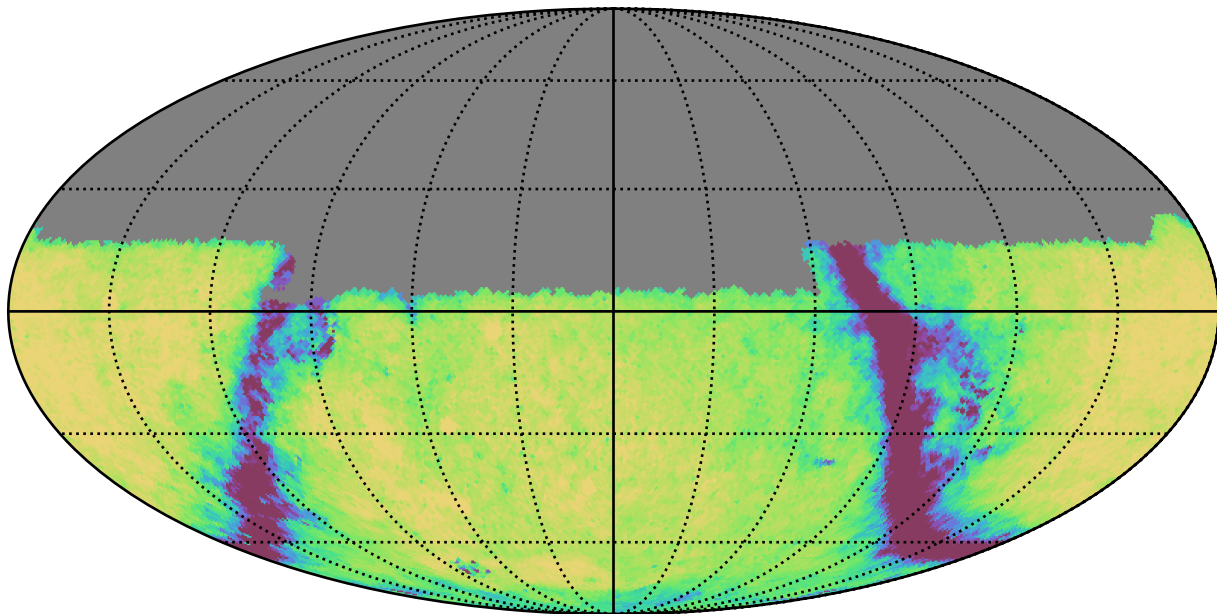
smc_lmc_v3.3_10yrs Yr 1 u band: Exgal_CoaddM5
