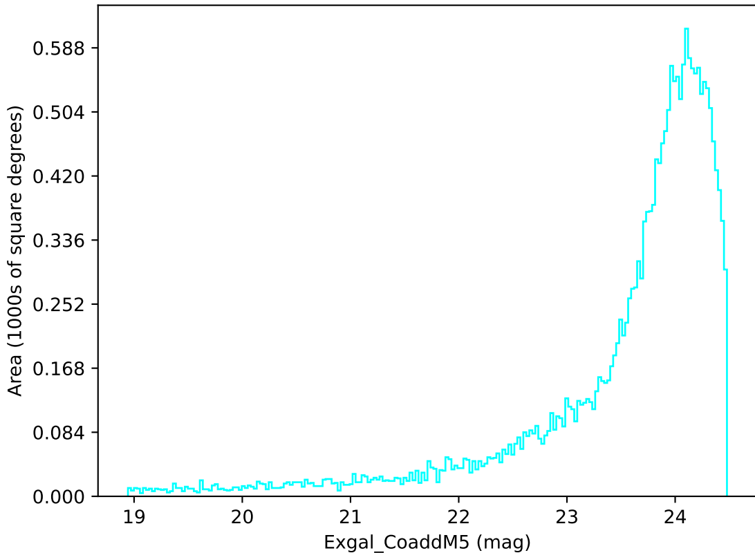
smc_lmc_v3.3_10yrs Yr 1 u band: Exgal_CoaddM5
