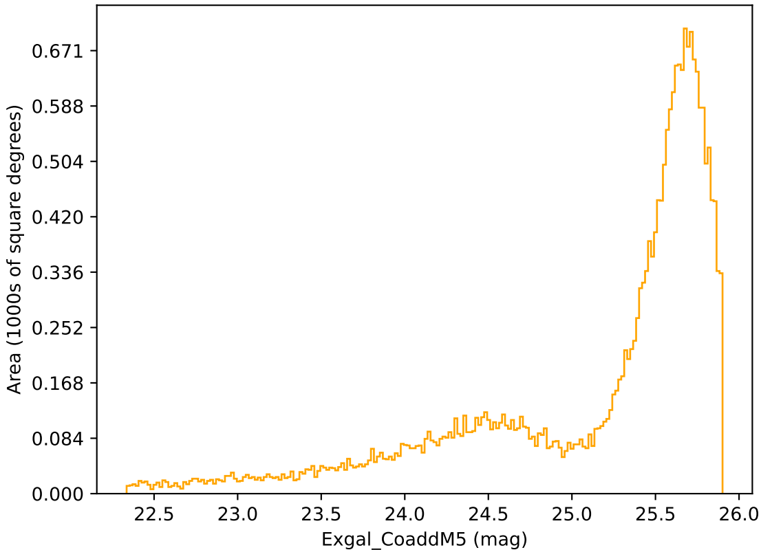
smc_lmc_v3.3_10yrs Yr 1 r band: Exgal_CoaddM5
