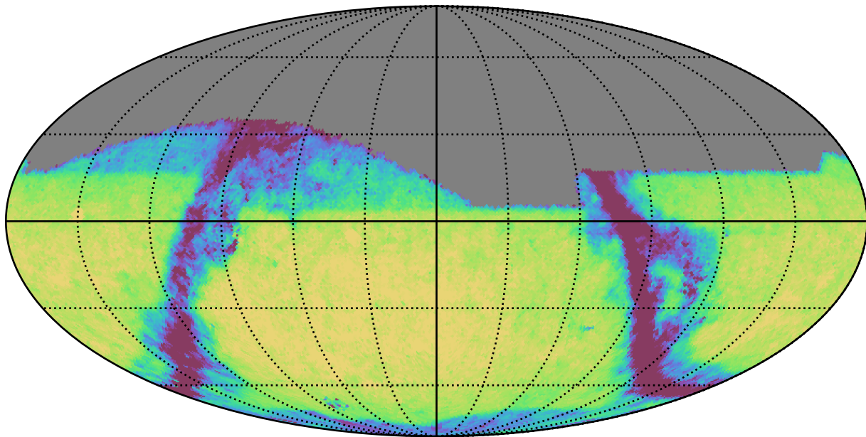
smc_lmc_v3.3_10yrs Yr 1 i band: Exgal_CoaddM5
