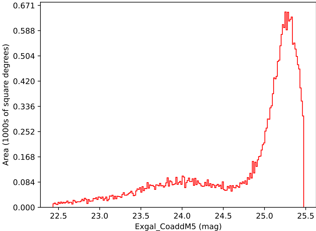
smc_lmc_v3.3_10yrs Yr 1 i band: Exgal_CoaddM5
