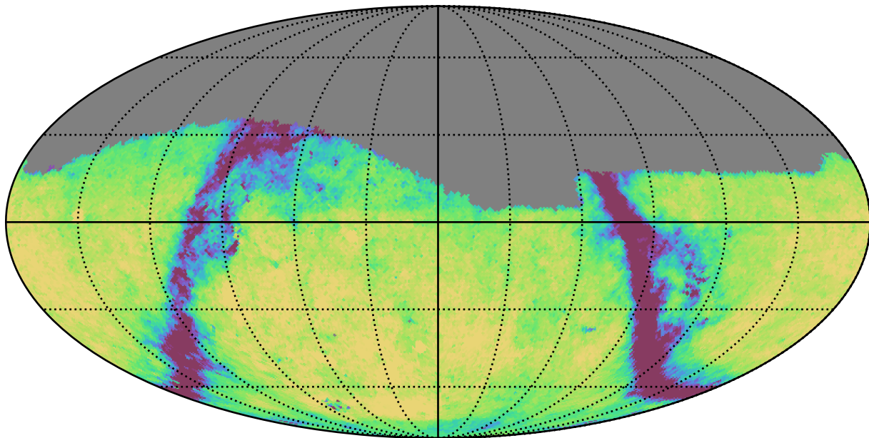
smc_lmc_v3.3_10yrs Yr 1 g band: Exgal_CoaddM5
