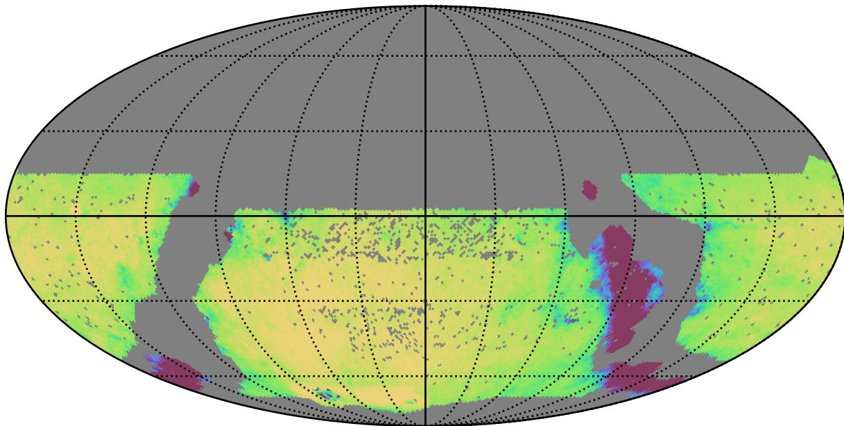
smc_lmc_v3.3_10yrs WFD u band: Exgal_CoaddM5
