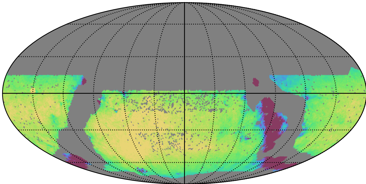
smc_lmc_v3.3_10yrs WFD i band: Exgal_CoaddM5
