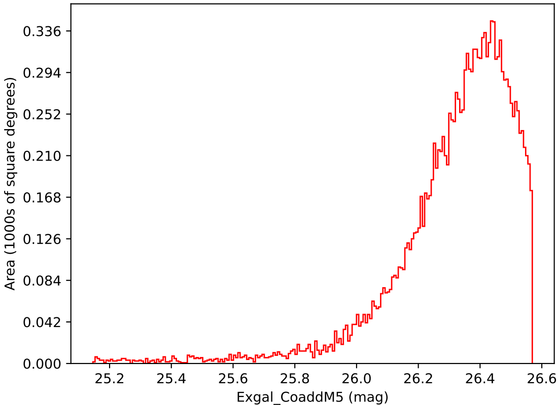
smc_lmc_v3.3_10yrs WFD i band: Exgal_CoaddM5
