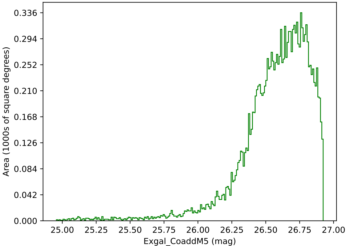
smc_lmc_v3.3_10yrs WFD g band: Exgal_CoaddM5
